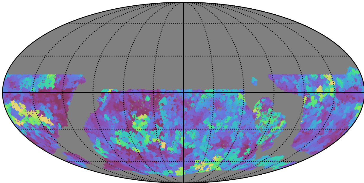
ddf_loaded_half_fl8_v3.4_10yrs WFD g band: Max seeingEff
