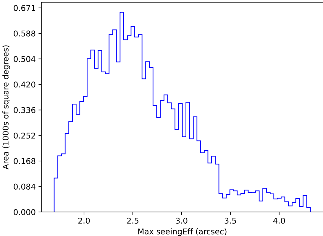
ddf_loaded_half_fl8_v3.4_10yrs WFD g band: Max seeingEff
