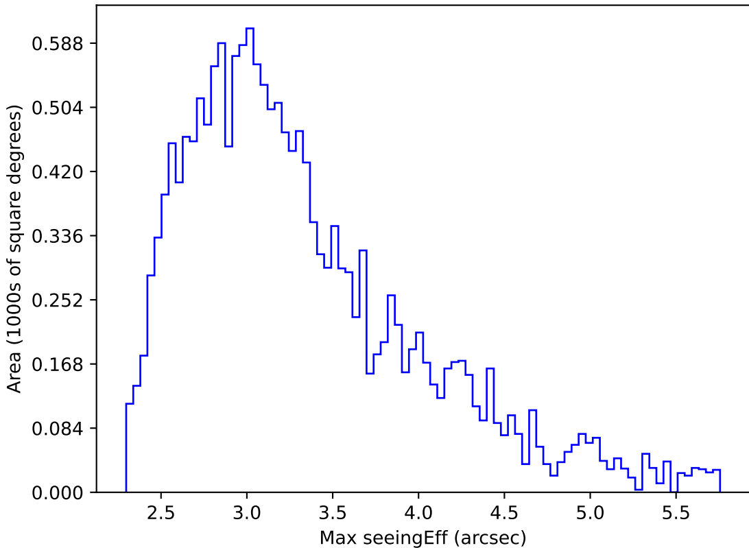
ddf_loaded_half_fl8_v3.4_10yrs WFD all bands: Max seeingEff
