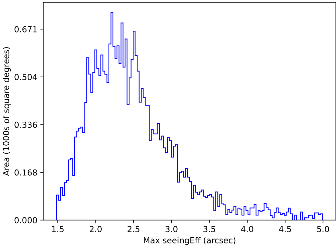
ddf_loaded_half_fl8_v3.4_10yrs All sky z band: Max seeingEff
