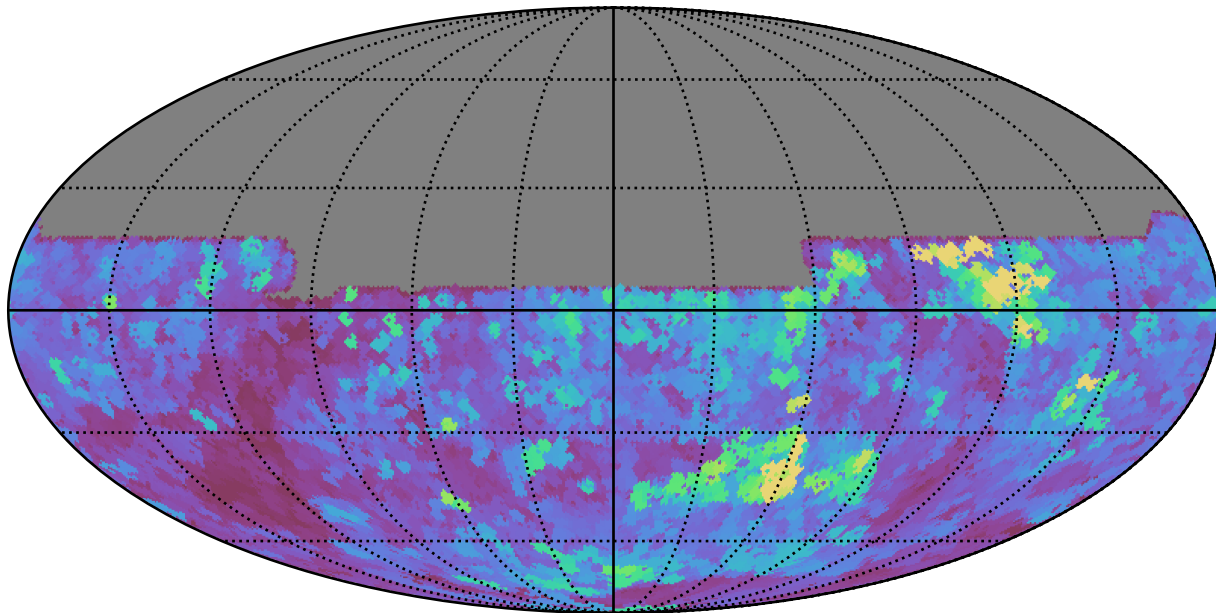
ddf_loaded_half_fl8_v3.4_10yrs All sky y band: Max seeingEff
