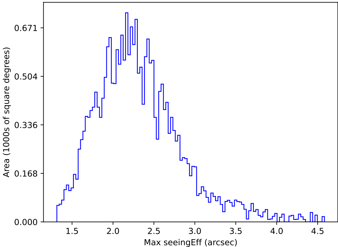
ddf_loaded_half_fl8_v3.4_10yrs All sky y band: Max seeingEff
