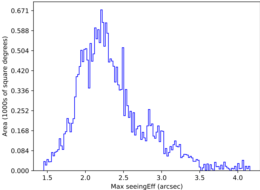
ddf_loaded_half_f18_v3.4_10yrs All sky u band: Max seeingEff
