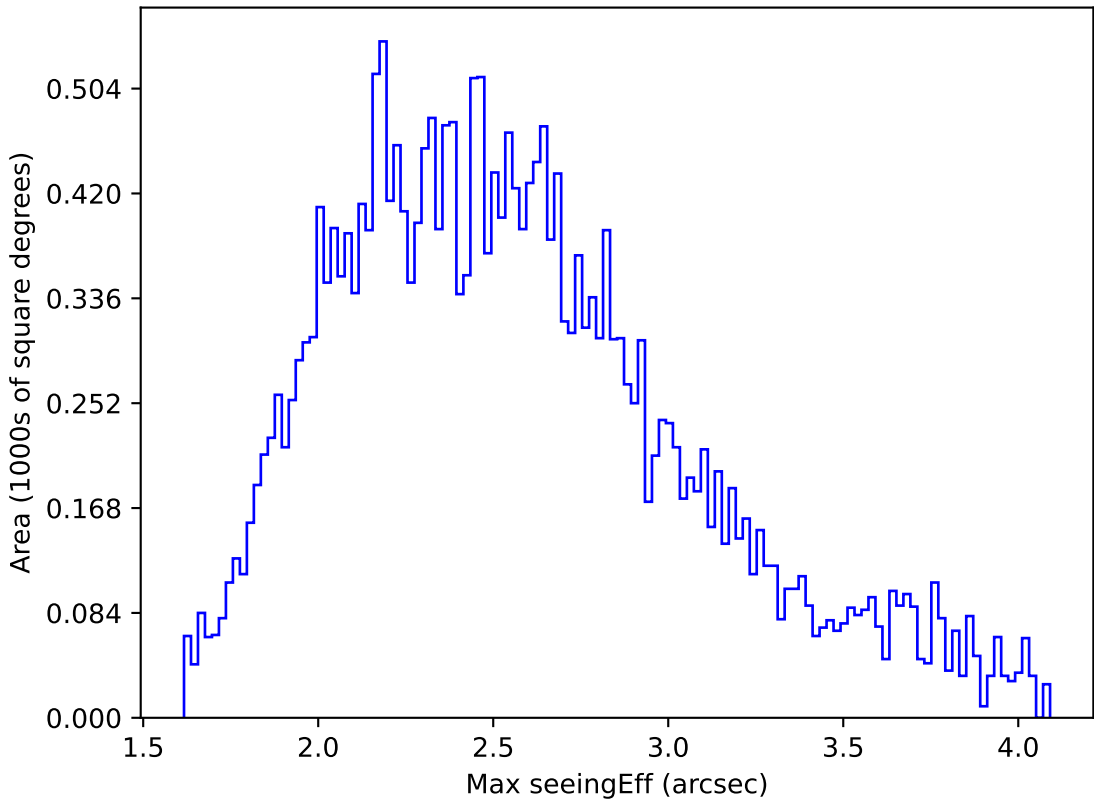
ddf_loaded_half_fl8_v3.4_10yrs All sky r band: Max seeingEff
