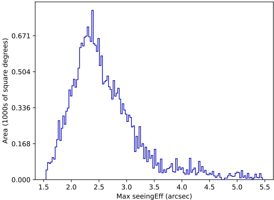
ddf_loaded_half_fl8_v3.4_10yrs All sky i band: Max seeingEff
