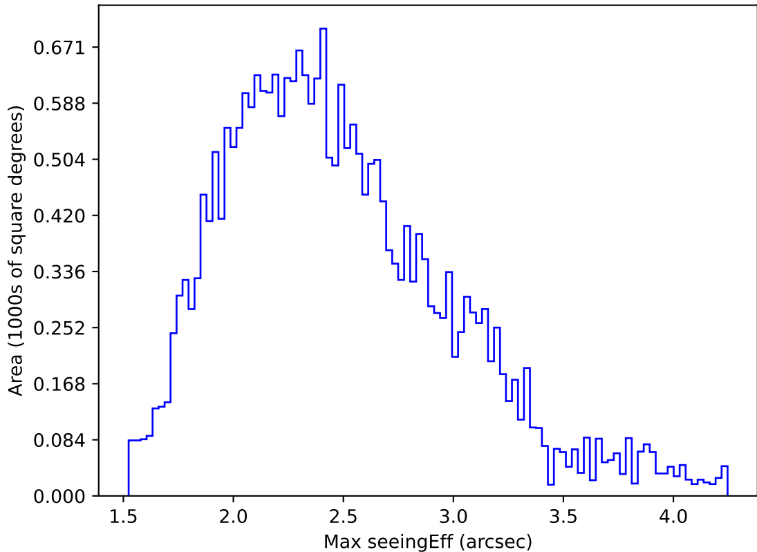
ddf_loaded_half_fl8_v3.4_10yrs All sky g band: Max seeingEff
