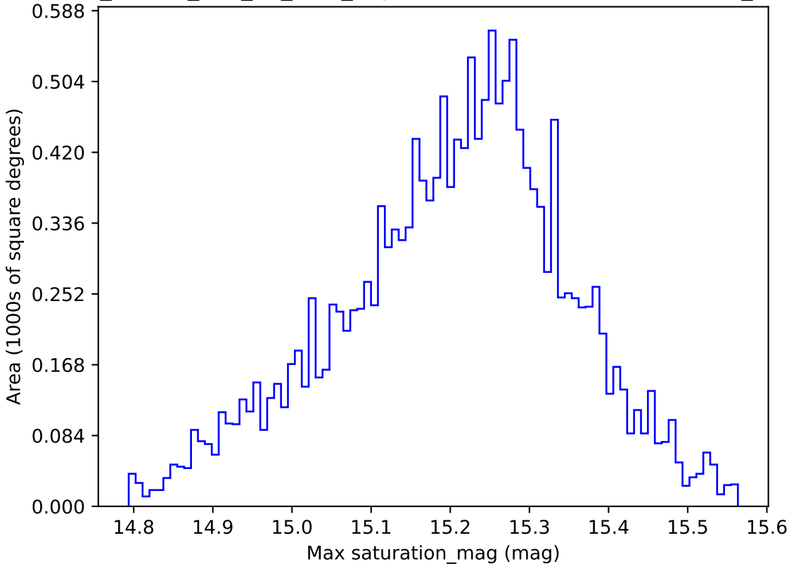
ddf_loaded_half_fl8_v3.4_10yrs WFD z band: Max saturation_mag
