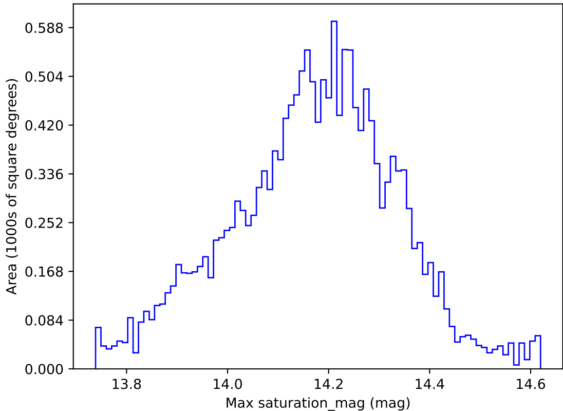
ddf_loaded_half_fl8_v3.4_10yrs WFD y band: Max saturation_mag
