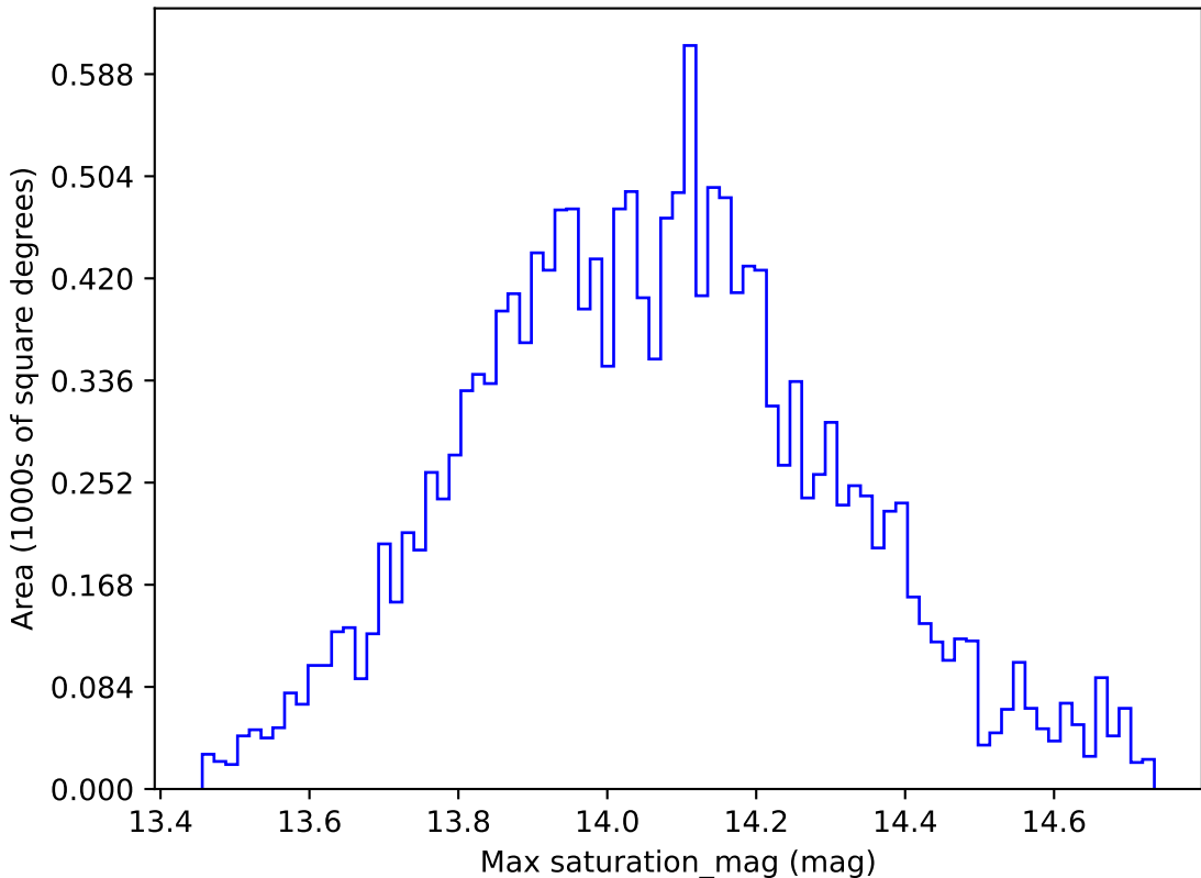
ddf_loaded_half_fl8_v3.4_10yrs WFD u band: Max saturation_mag
