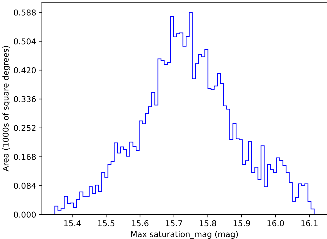
ddf_loaded_half_fl8_v3.4_10yrs WFD r band: Max saturation_mag
