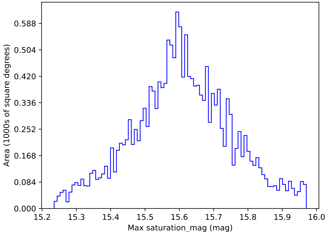
ddf_loaded_half_fl8_v3.4_10yrs WFD i band: Max saturation_mag
