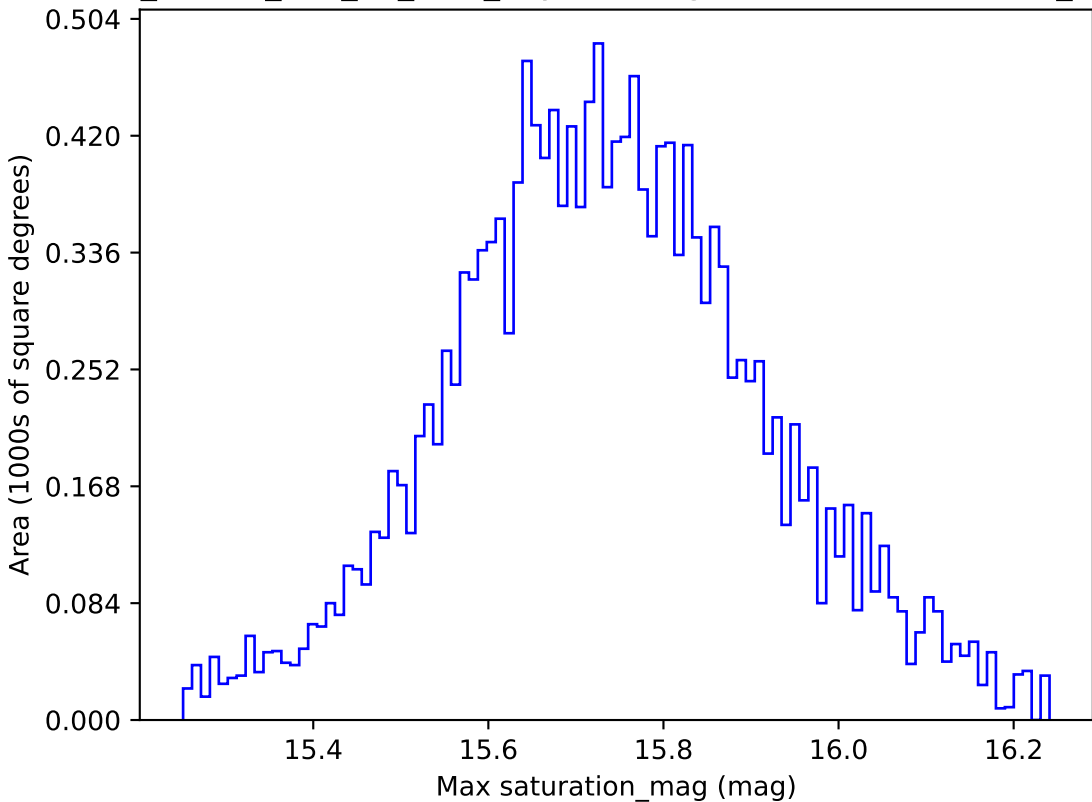
ddf_loaded_half_fl8_v3.4_10yrs WFD g band: Max saturation_mag
