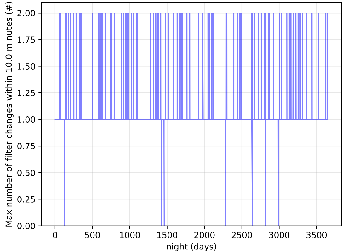
ddf_loaded_half_fl8_v3.4_10yrs Per Night: Max number of filter changes within 10.0 minutes
