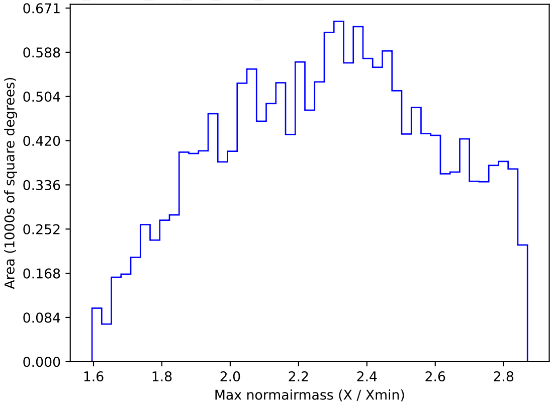
ddf_loaded_half_fl8_v3.4_10yrs WFD z band: Max normairmass
