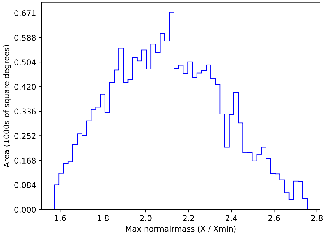
ddf_loaded_half_fl8_v3.4_10yrs WFD y band: Max normairmass
