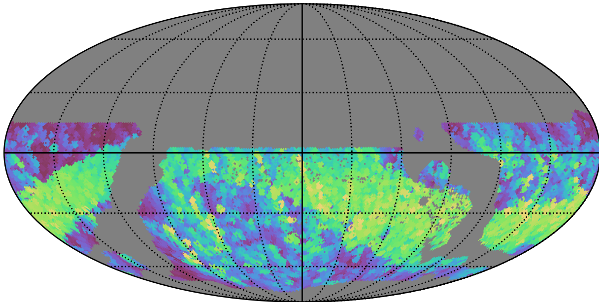
ddf_loaded_half_fl8_v3.4_10yrs WFD r band: Max normairmass
