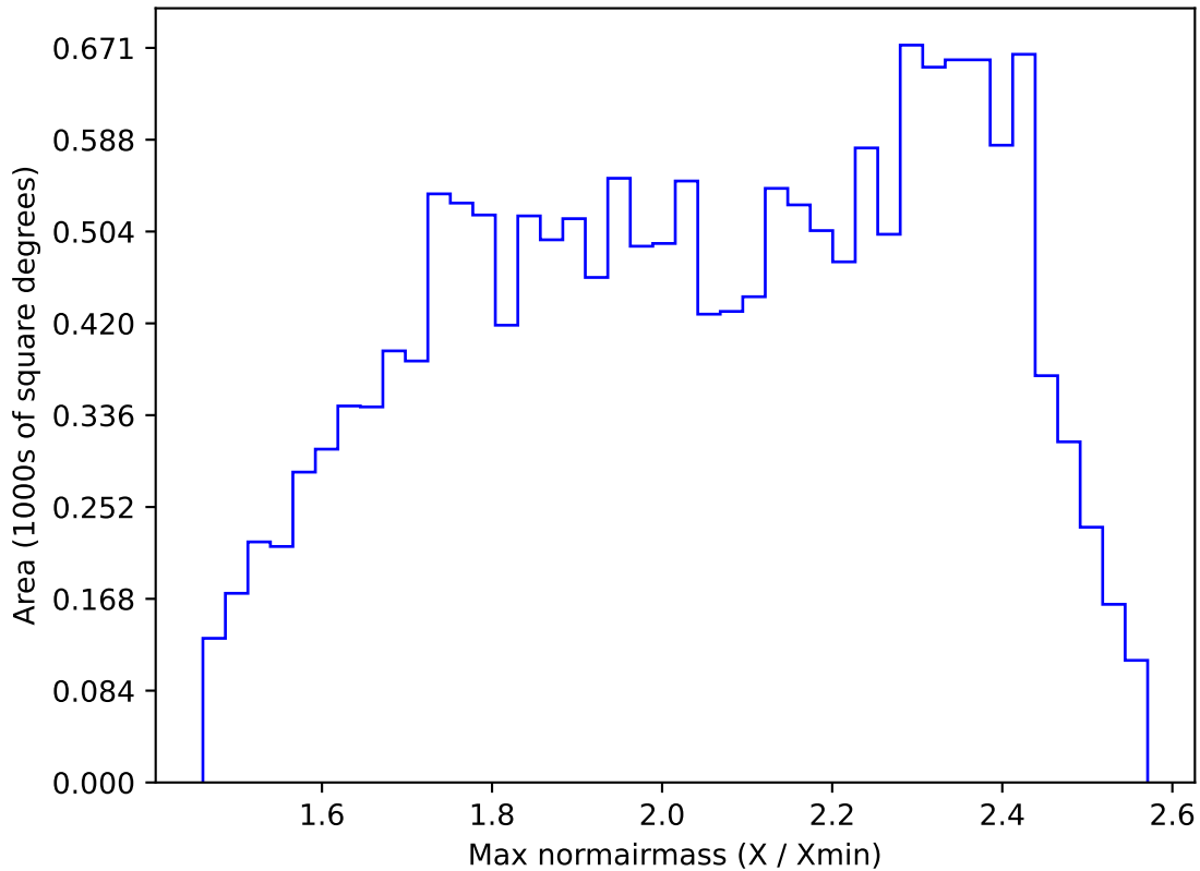
ddf_loaded_half_fl8_v3.4_10yrs WFD r band: Max normairmass
