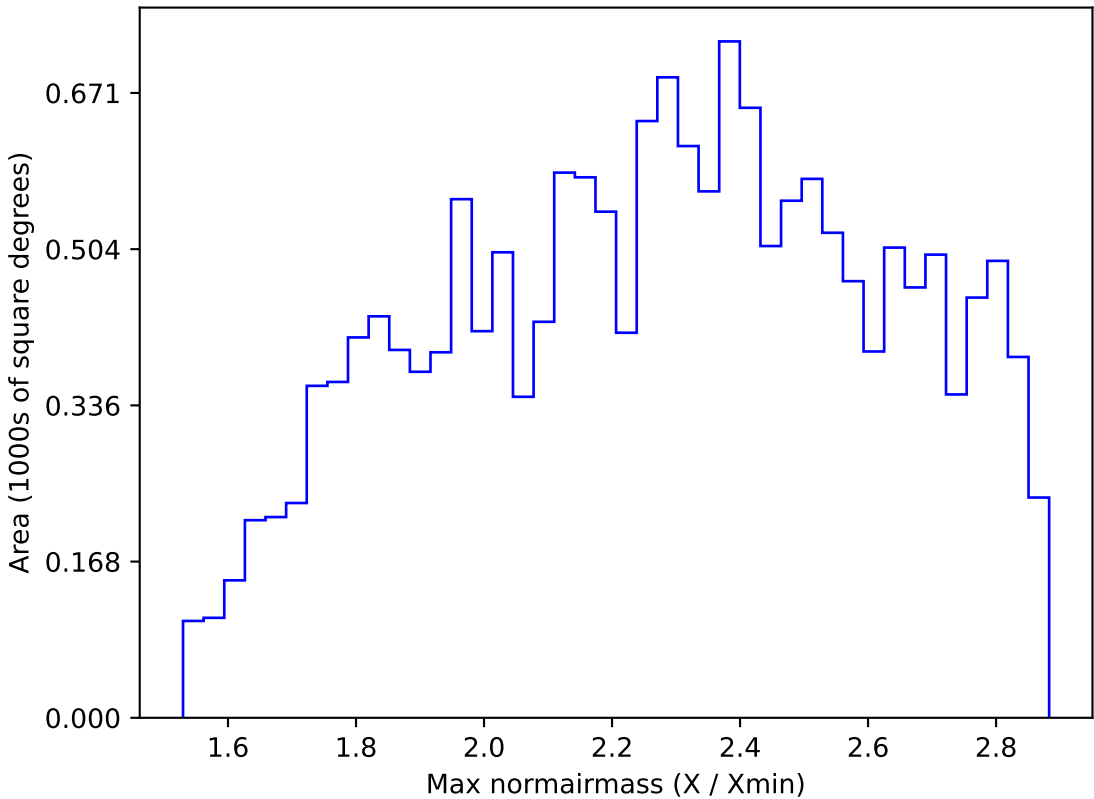
ddf_loaded_half_fl8_v3.4_10yrs WFD i band: Max normairmass
