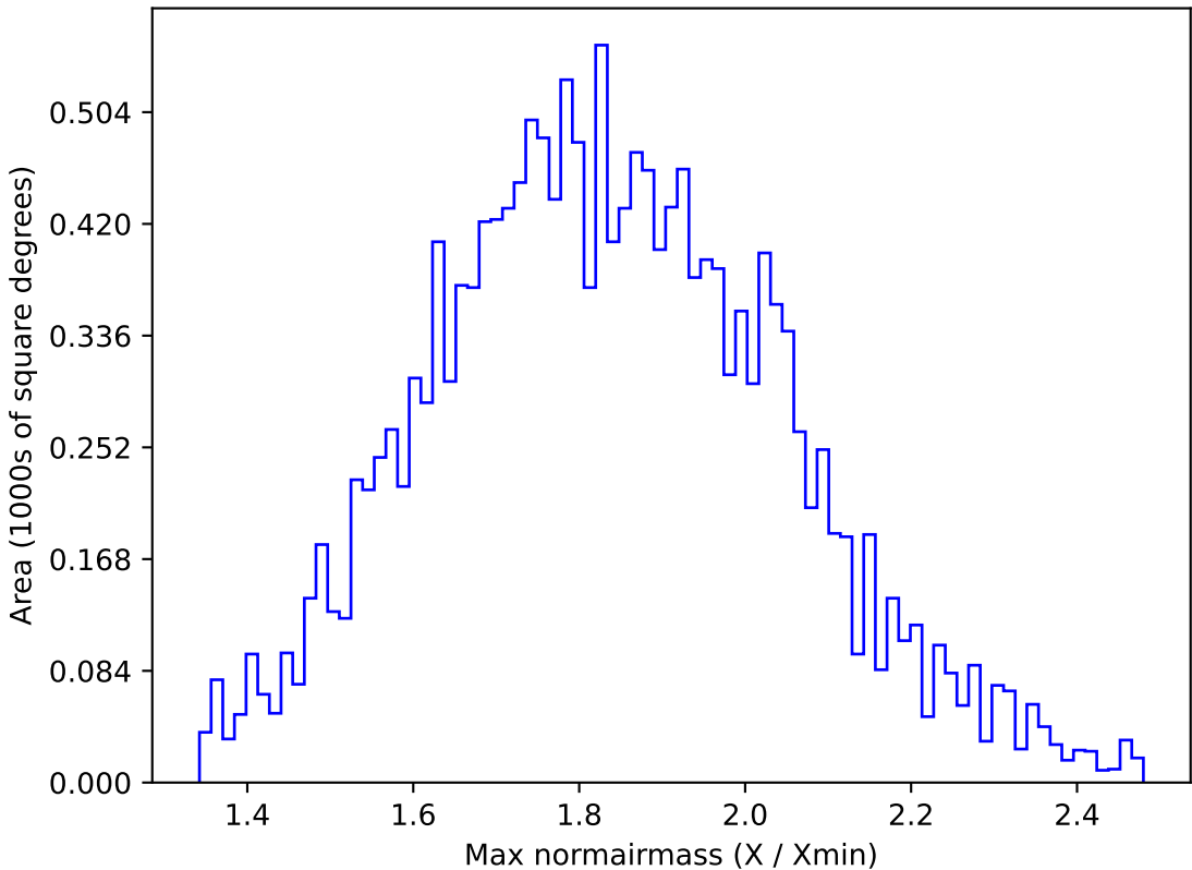
ddf_loaded_half_fl8_v3.4_10yrs WFD g band: Max normairmass
