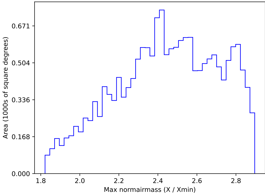
ddf_loaded_half_fl8_v3.4_10yrs WFD all bands: Max normairmass
