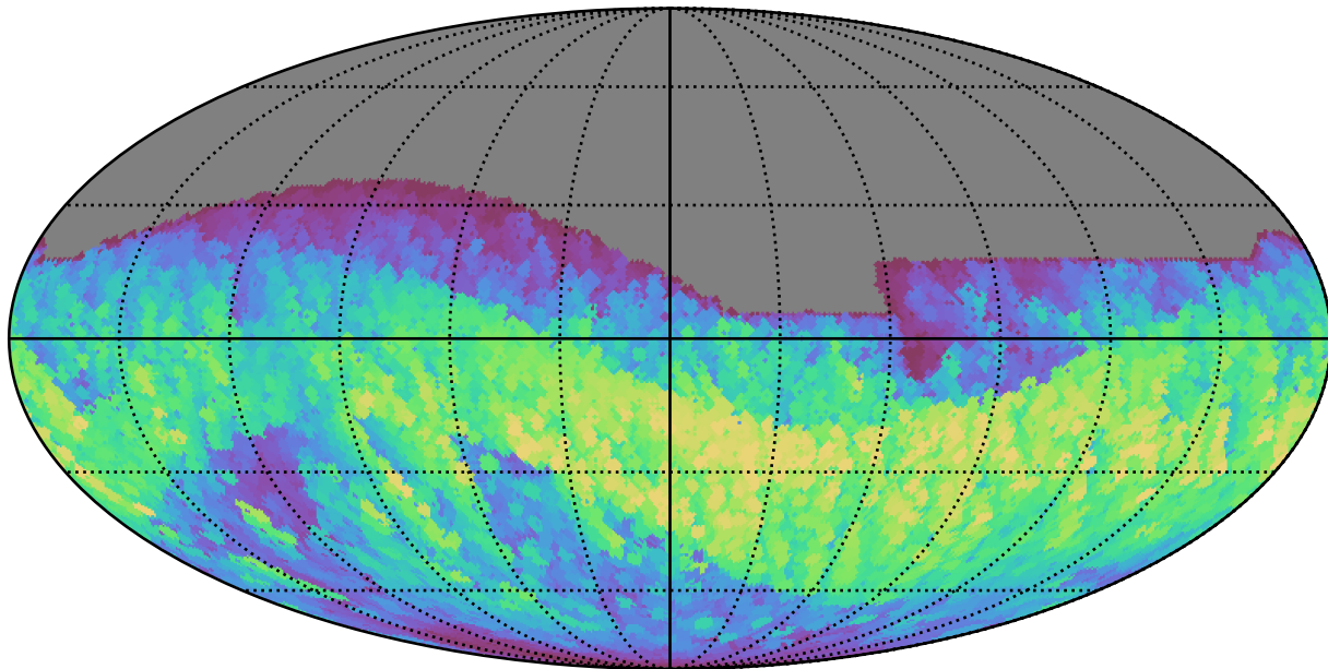
ddf_loaded_half_fl8_v3.4_10yrs All sky z band: Max normairmass
