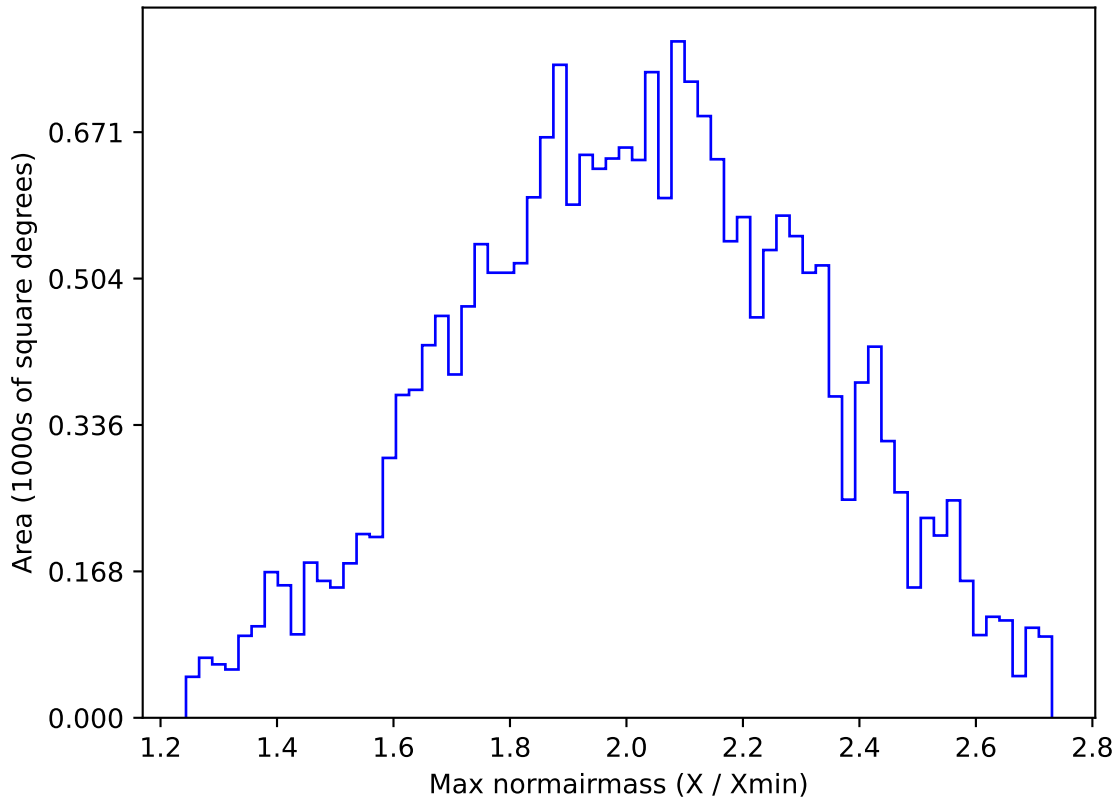
ddf_loaded_half_fl8_v3.4_10yrs All sky y band: Max normairmass
