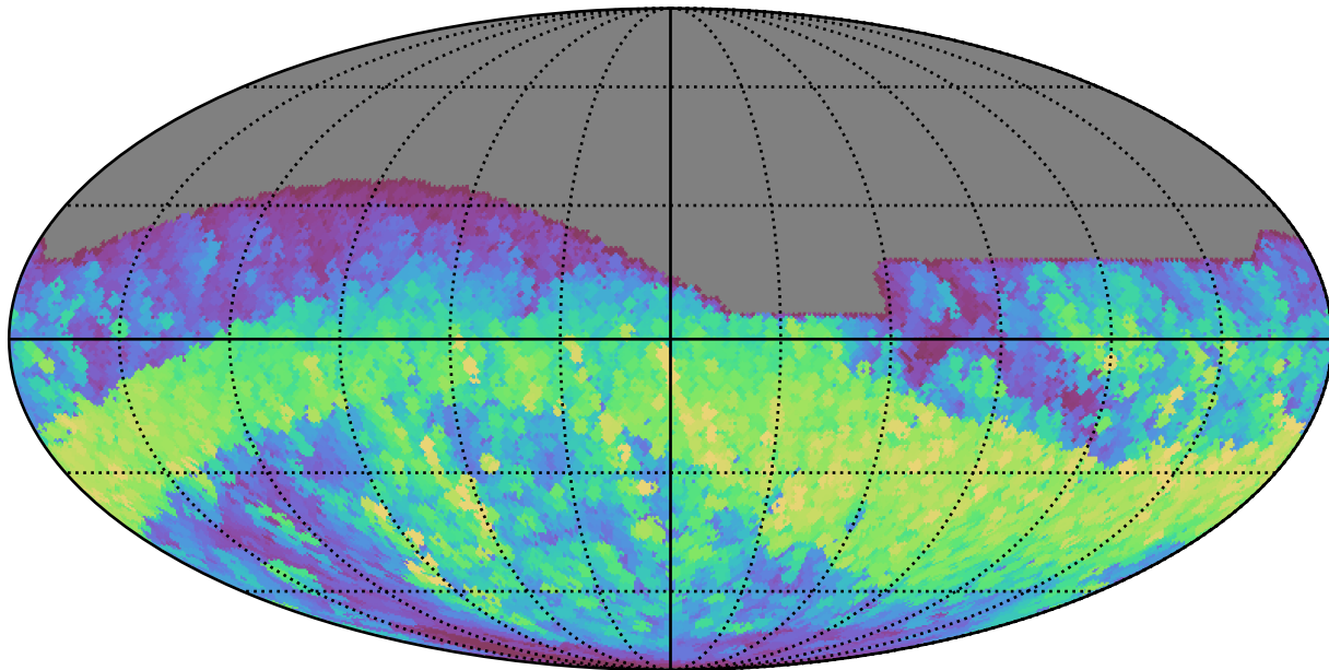
ddf_loaded_half_fl8_v3.4_10yrs All sky r band: Max normairmass
