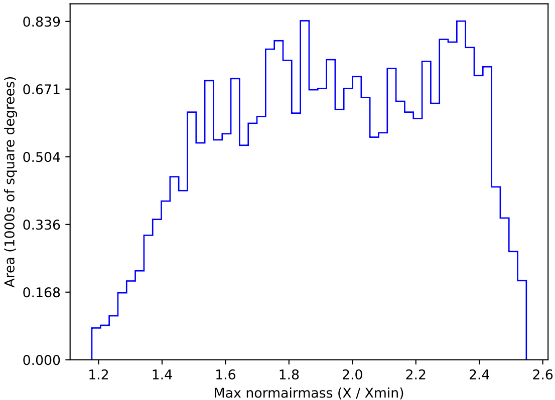
ddf_loaded_half_fl8_v3.4_10yrs All sky r band: Max normairmass
