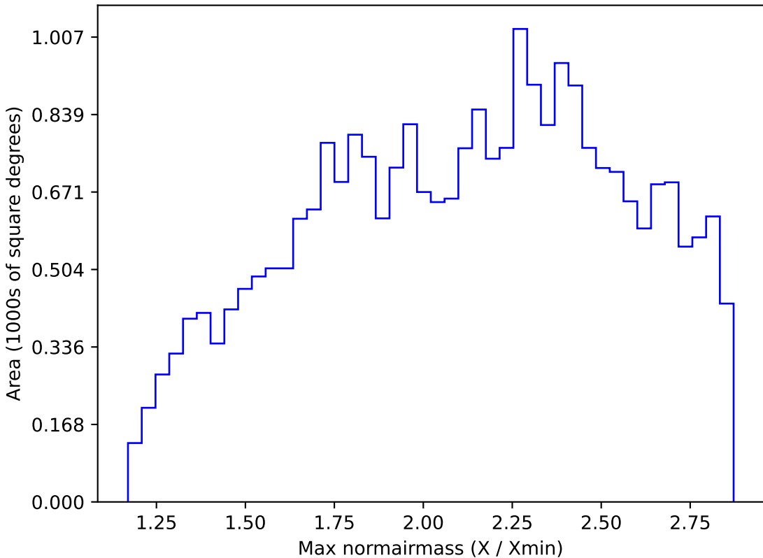
ddf_loaded_half_fl8_v3.4_10yrs All sky i band: Max normairmass
