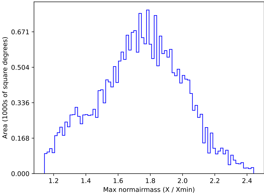
ddf_loaded_half_fl8_v3.4_10yrs All sky g band: Max normairmass
