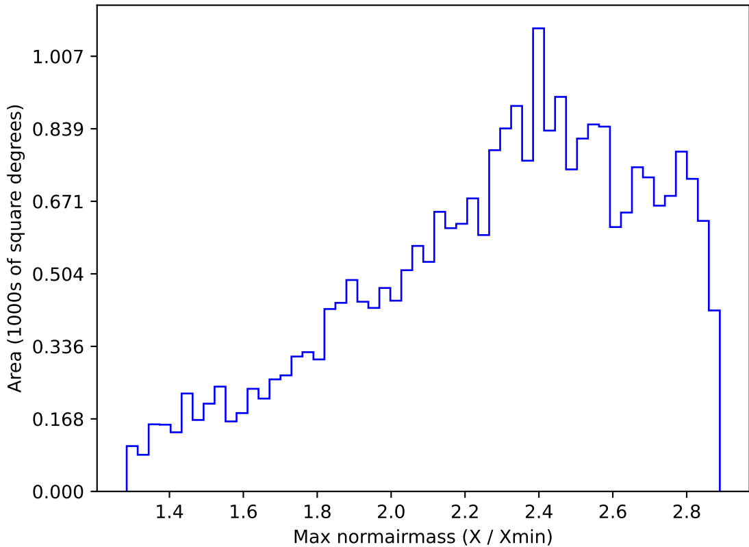
ddf_loaded_half_fl8_v3.4_10yrs All sky all bands: Max normairmass
