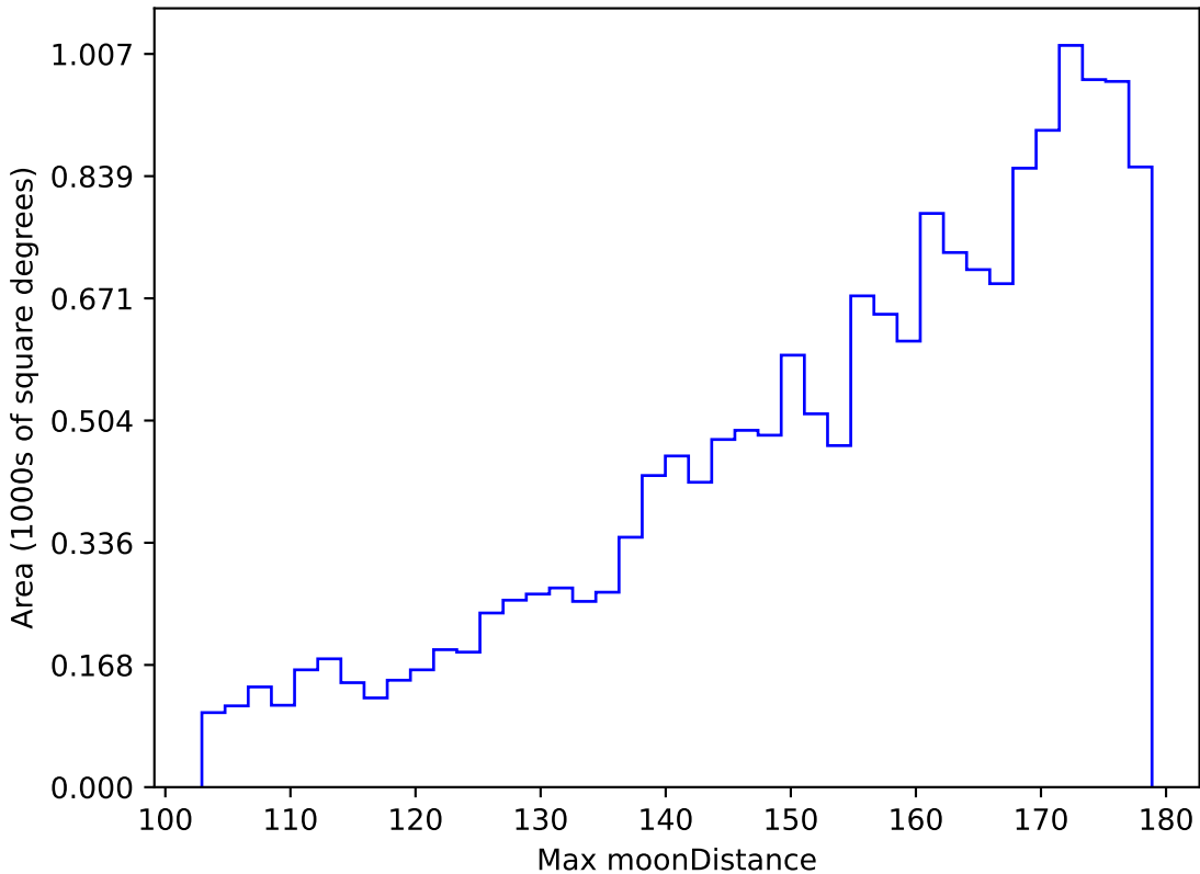
ddf_loaded_half_fl8_v3.4_10yrs WFD z band: Max moonDistance
