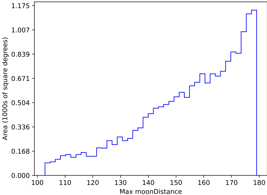
ddf_loaded_half_fl8_v3.4_10yrs WFD g band: Max moonDistance
