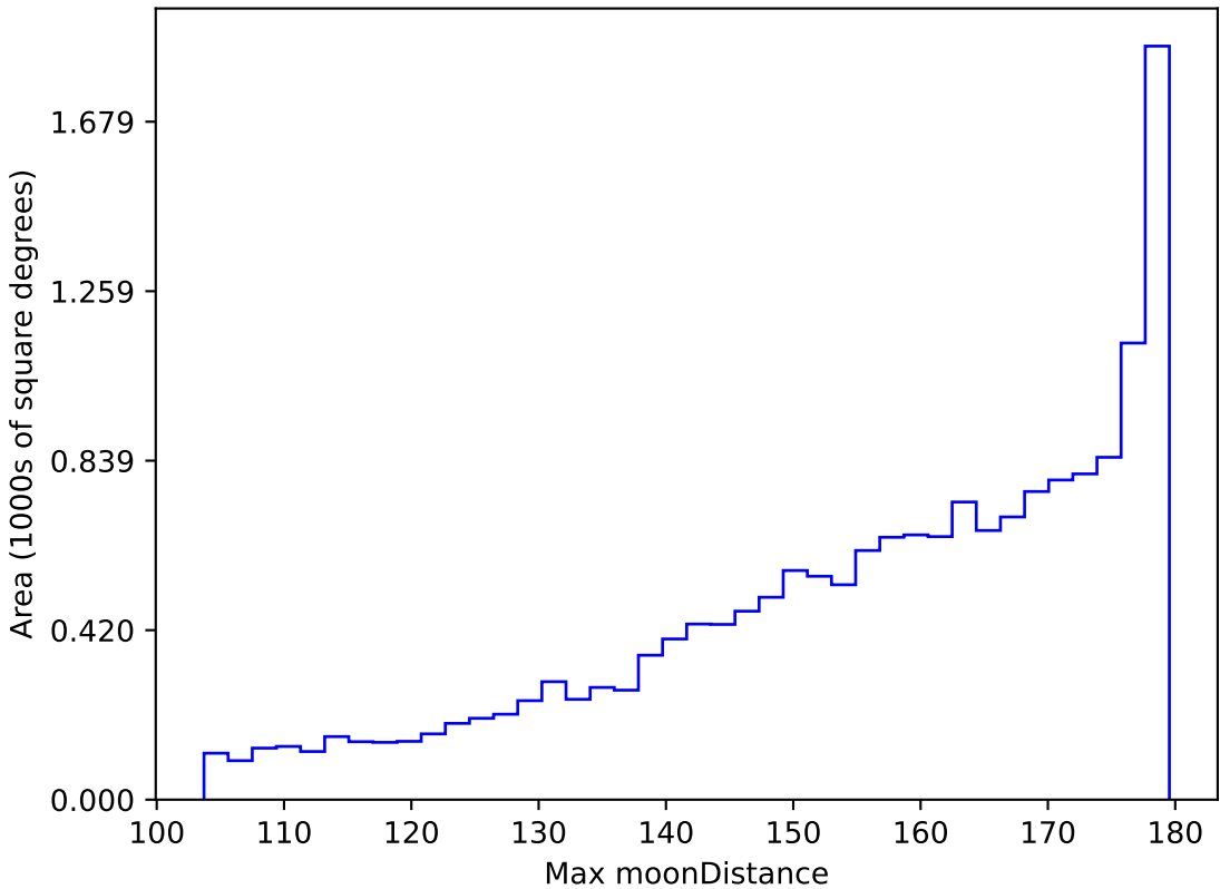
ddf_loaded_half_fl8_v3.4_10yrs WFD all bands: Max moonDistance
