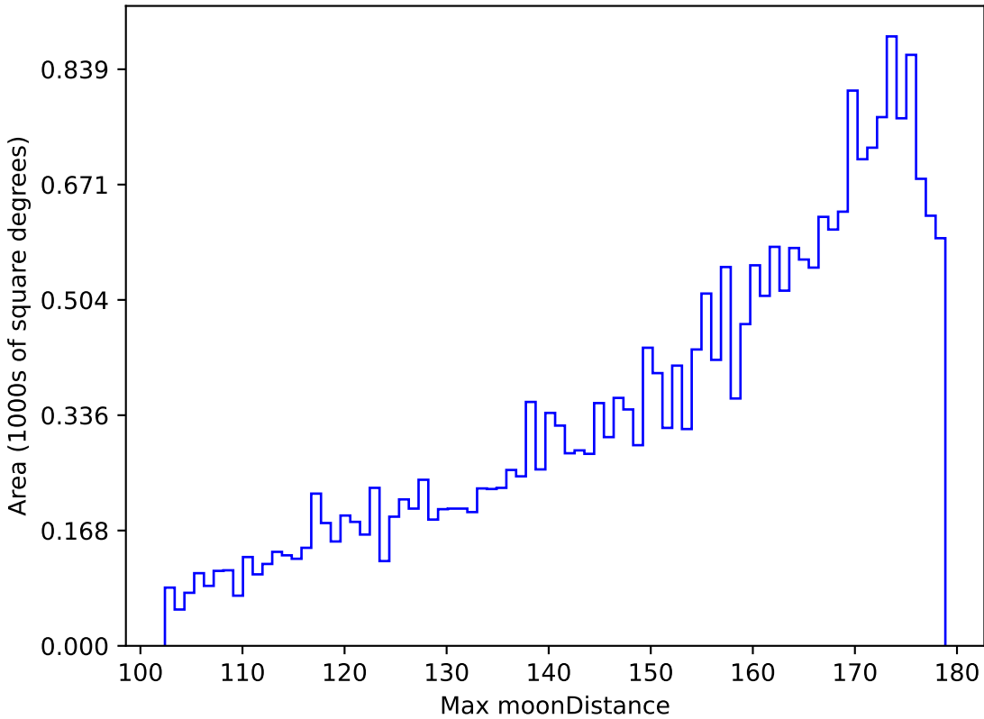
ddf_loaded_half_fl8_v3.4_10yrs All sky z band: Max moonDistance
