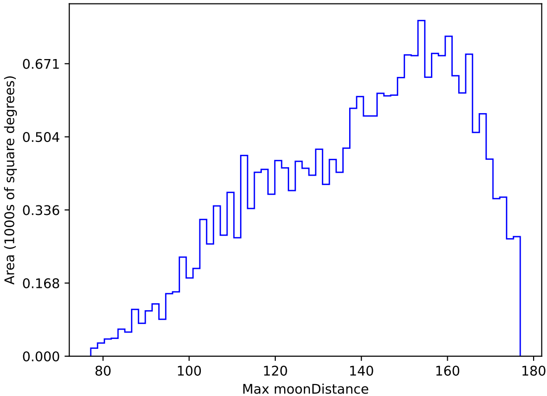
ddf_loaded_half_fl8_v3.4_10yrs All sky y band: Max moonDistance
