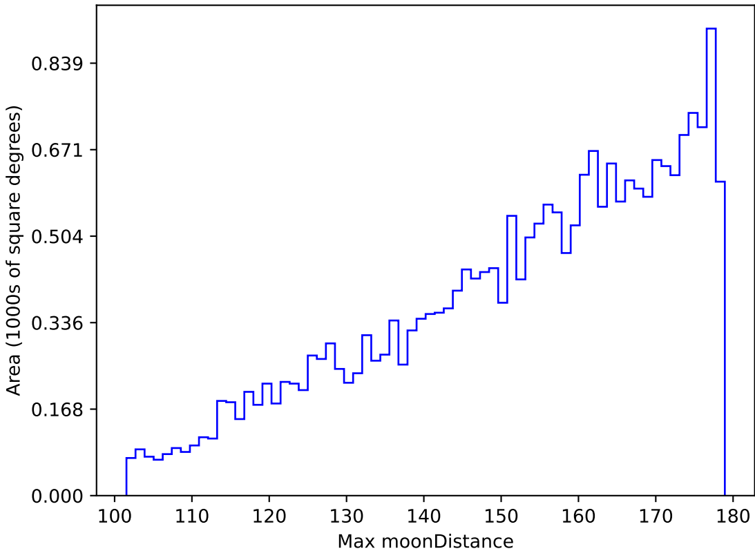
ddf_loaded_half_fl8_v3.4_10yrs All sky u band: Max moonDistance
