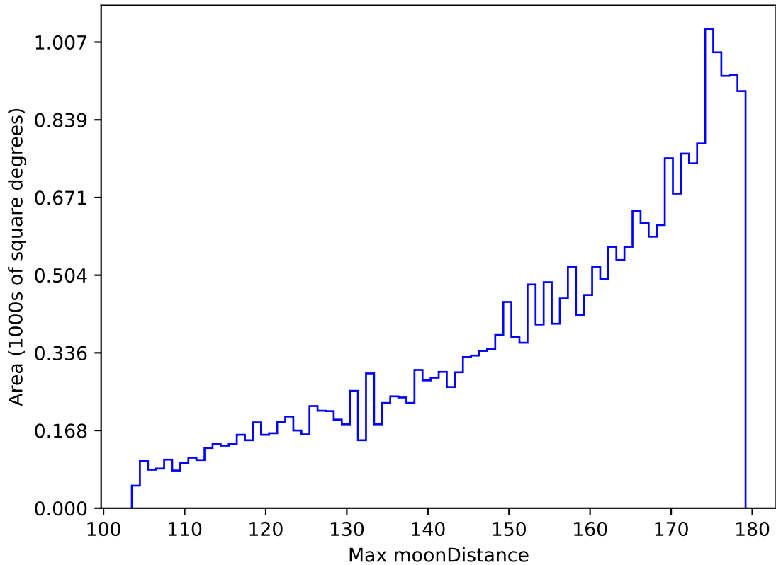
ddf_loaded_half_fl8_v3.4_10yrs All sky i band: Max moonDistance
