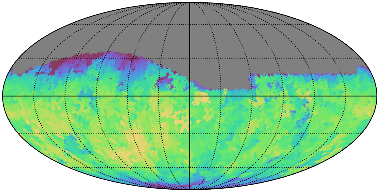
ddf_loaded_half_fl8_v3.4_10yrs Yr 1 z band: Max fiveSigmaDepth
