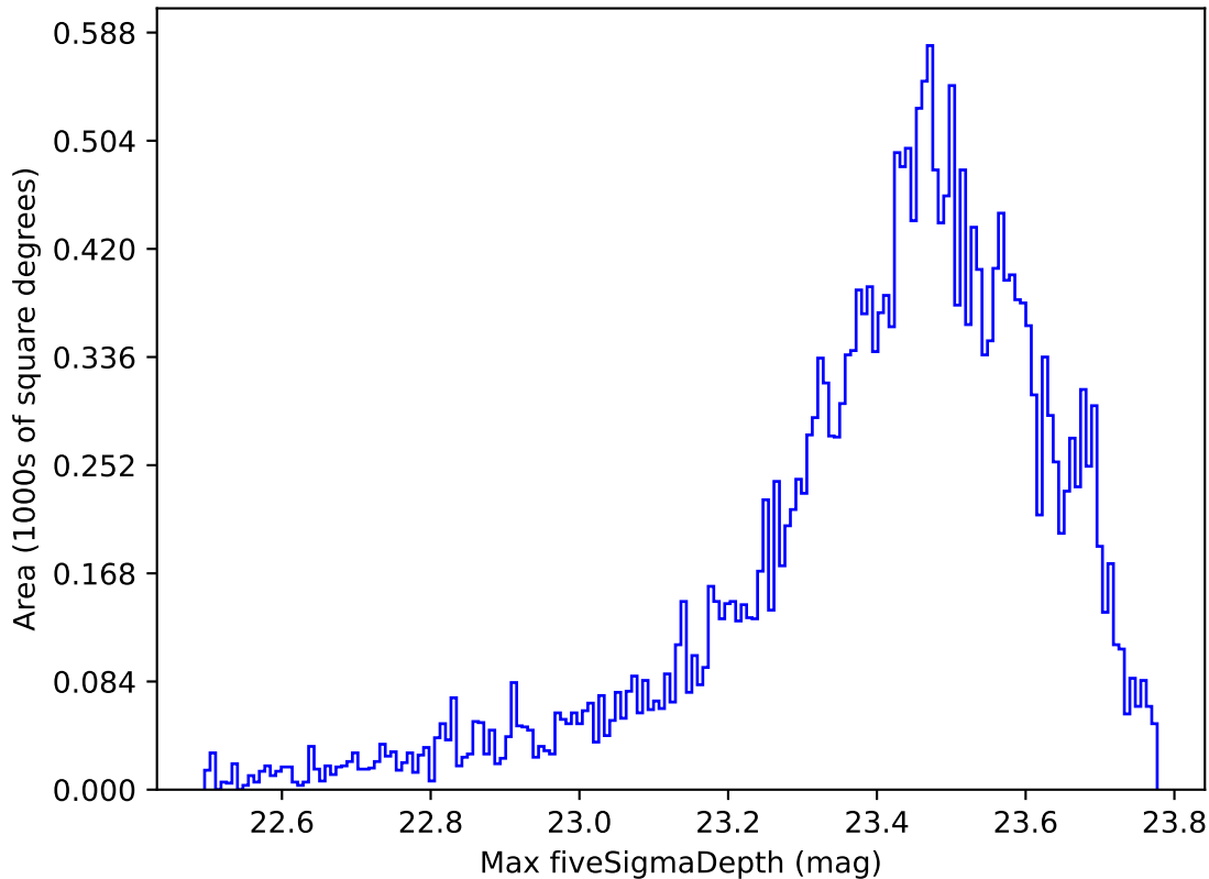
ddf_loaded_half_fl8_v3.4_10yrs Yr 1 z band: Max fiveSigmaDepth
