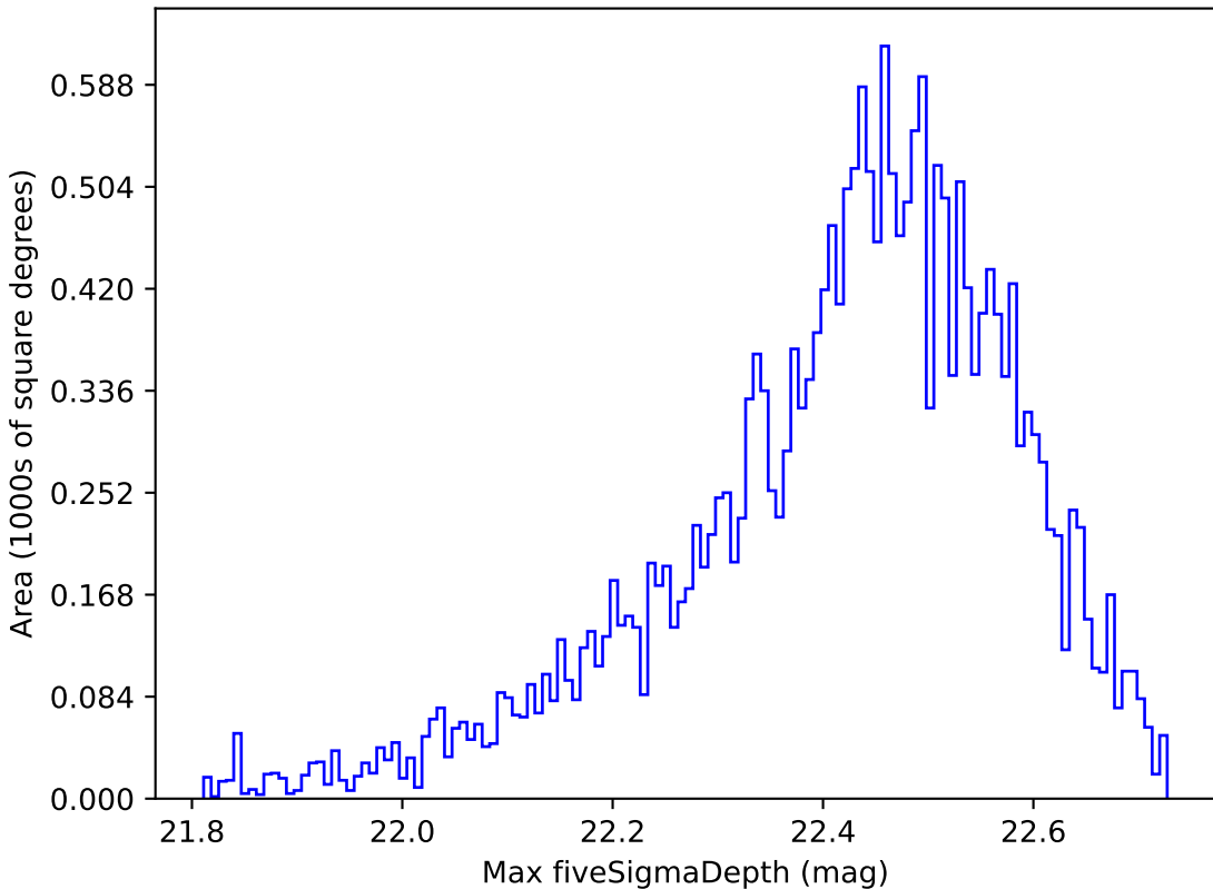
ddf_loaded_half_fl8_v3.4_10yrs Yr 1 y band: Max fiveSigmaDepth
