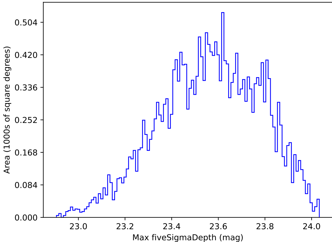
ddf_loaded_half_fl8_v3.4_10yrs Yr 1 u band: Max fiveSigmaDepth
