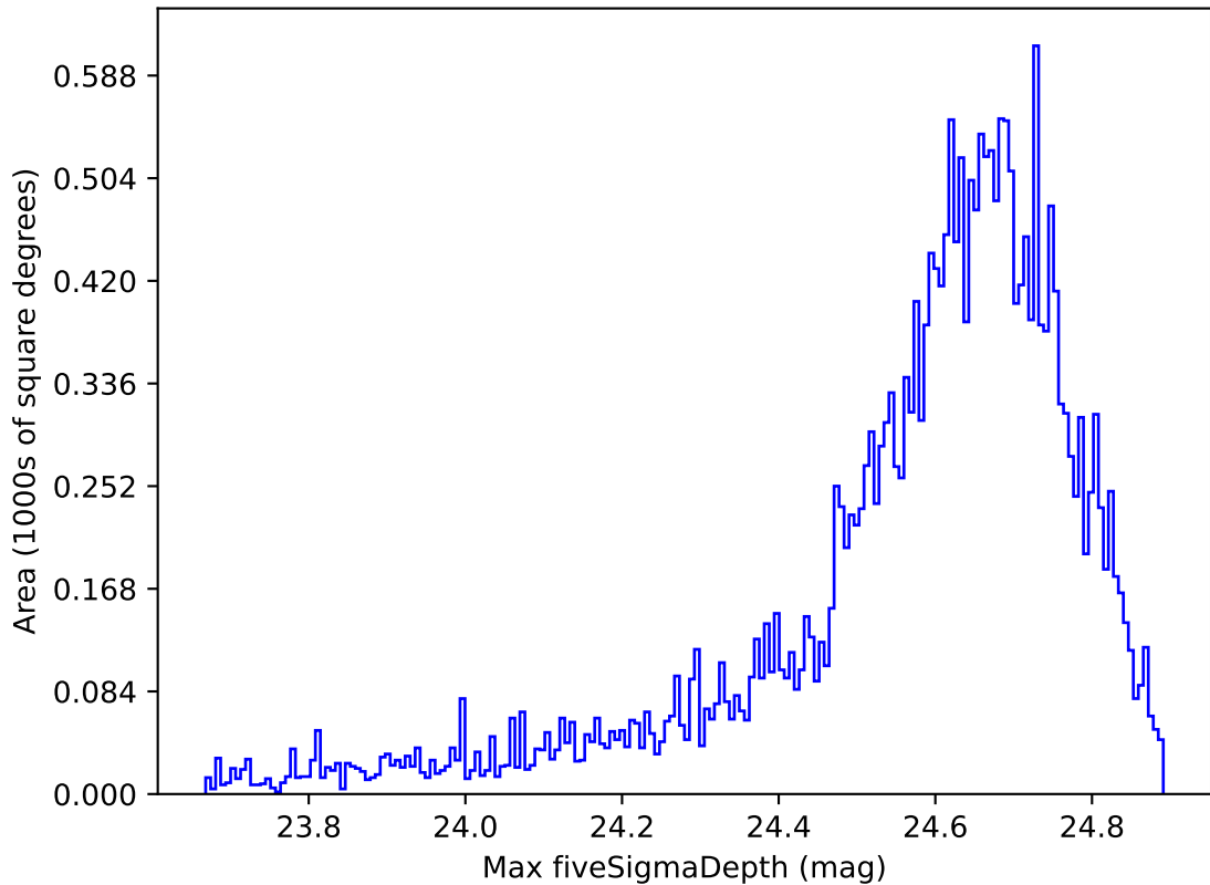
ddf_loaded_half_fl8_v3.4_10yrs Yr 1 r band: Max fiveSigmaDepth
