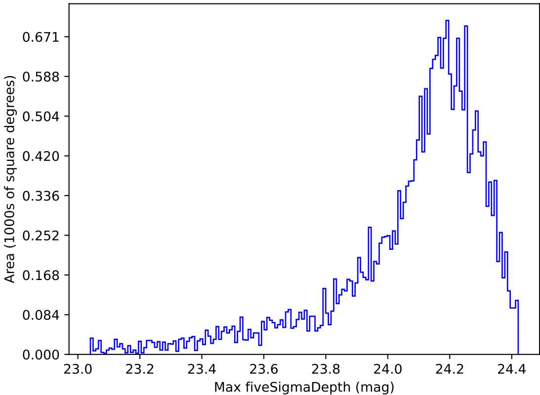
ddf_loaded_half_f18_v3.4_10yrs Yr 1 i band: Max fiveSigmaDepth
