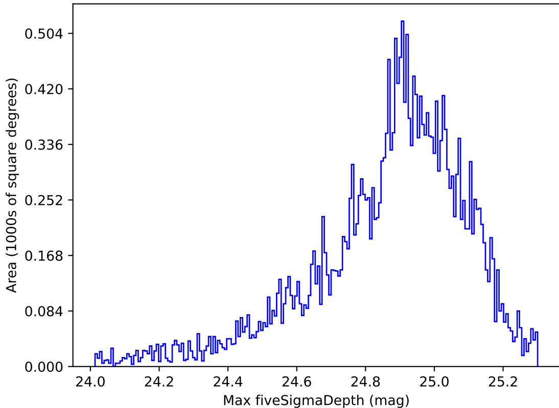
ddf_loaded_half_fl8_v3.4_10yrs Yr 1 g band: Max fiveSigmaDepth
