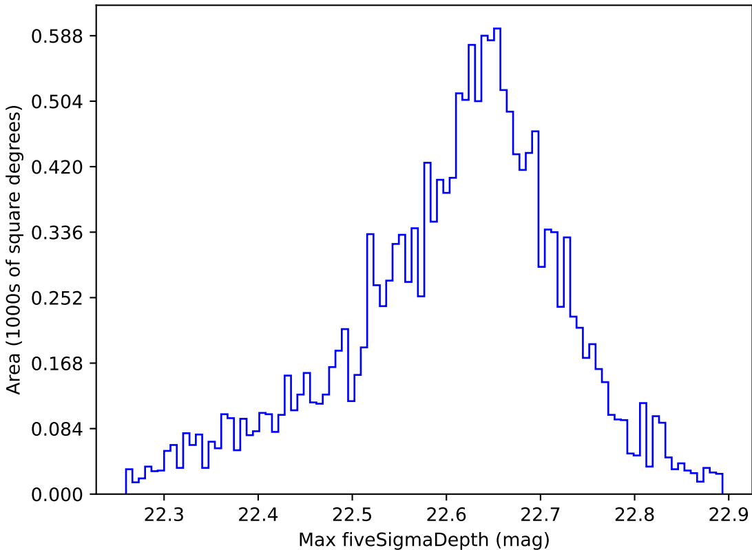
ddf_loaded_half_fl8_v3.4_10yrs WFD y band: Max fiveSigmaDepth
