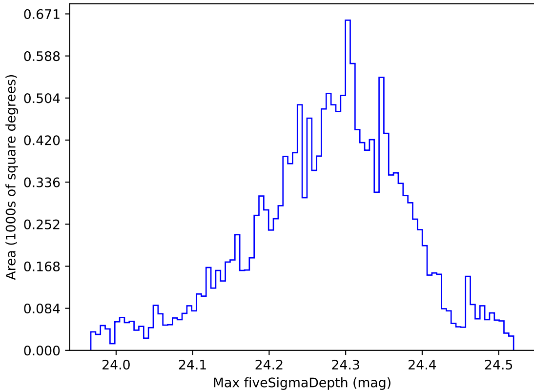
ddf_loaded_half_fl8_v3.4_10yrs WFD i band: Max fiveSigmaDepth
