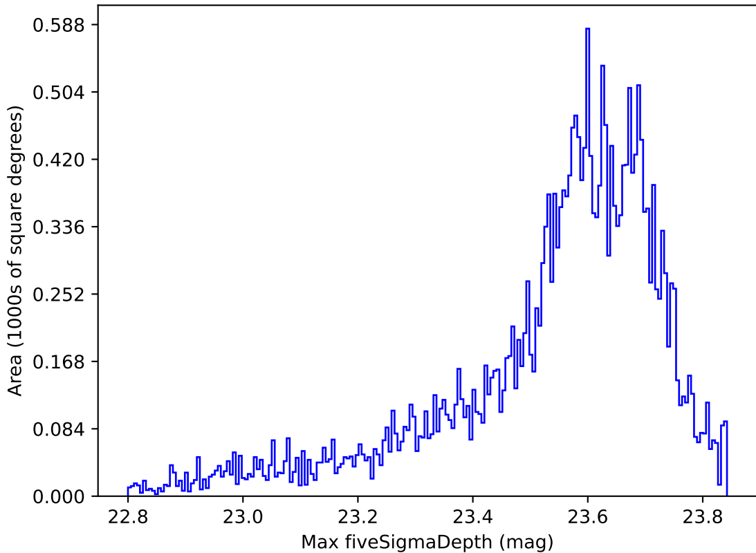
ddf_loaded_half_fl8_v3.4_10yrs All sky z band: Max fiveSigmaDepth
