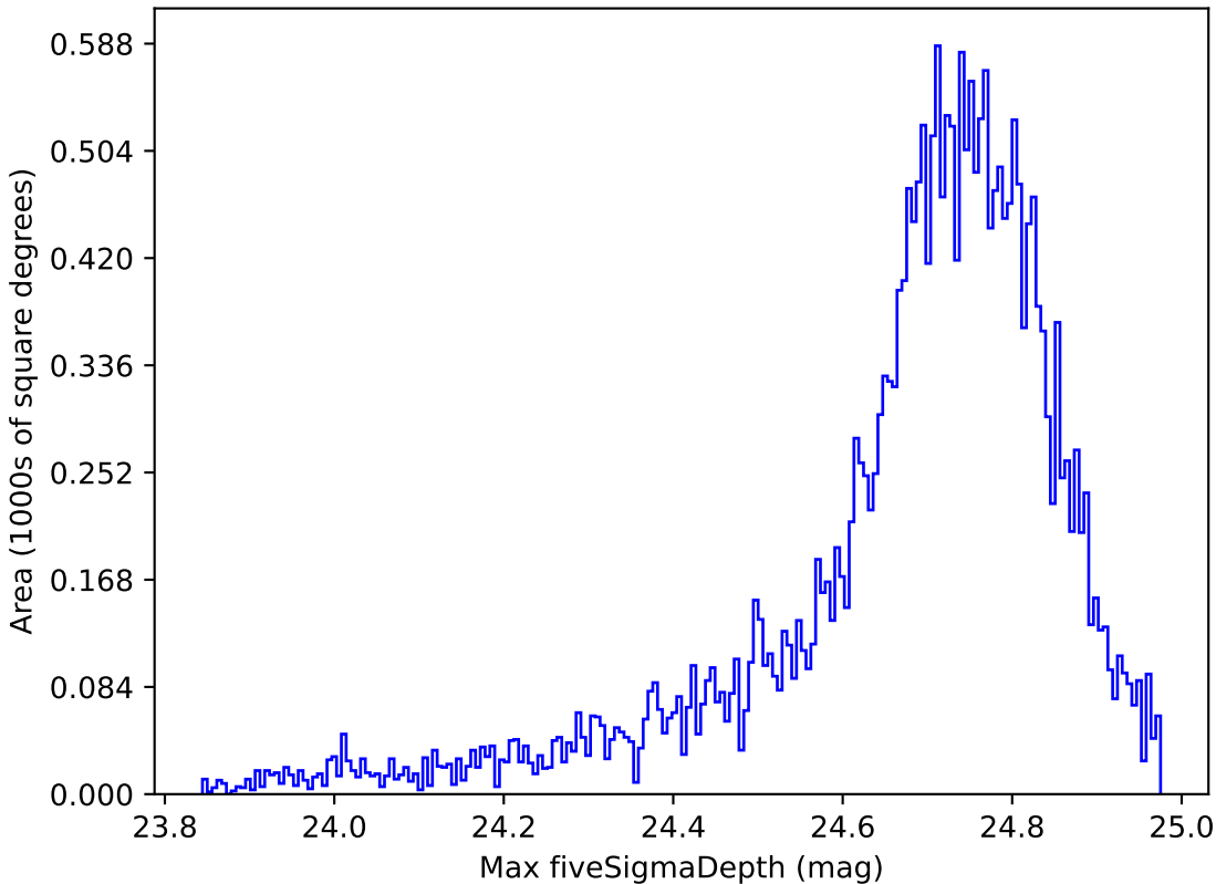
ddf_loaded_half_fl8_v3.4_10yrs All sky r band: Max fiveSigmaDepth
