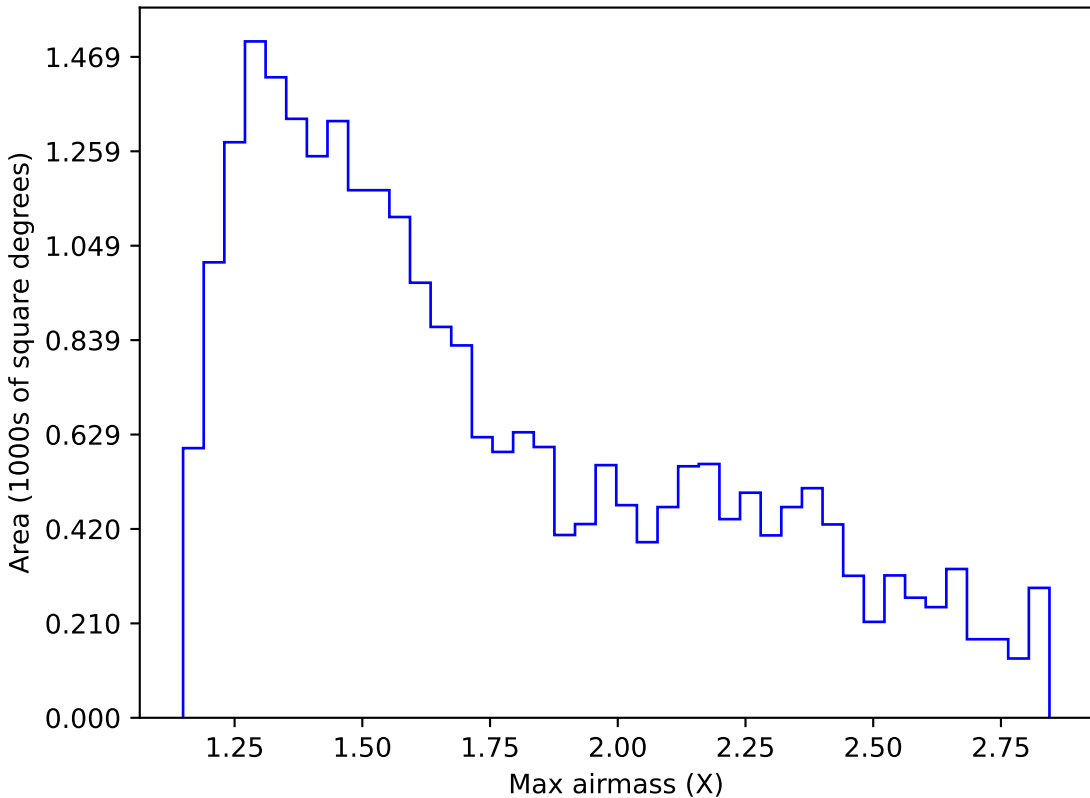
ddf_loaded_half_fl8_v3.4_10yrs Yr 1 z band: Max airmass
